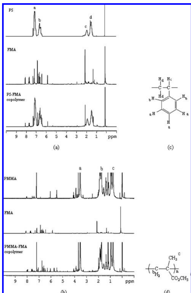
Figure 2. ^1\text{H} NMR spectra for (a) PS, FMA and PS-FMA copolymer, and (b) PMMA, FMA and PMMA-FMA copolymer, together with the structures and chemical shift assignments of (c) PS, and (d) PMMA.
